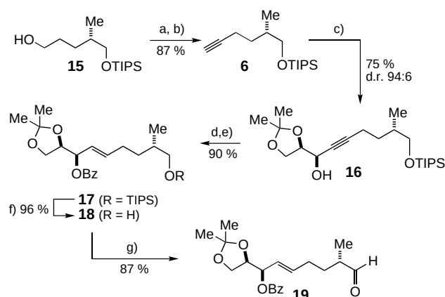
Scheme 3. a) TEMPO, bleach, KBr, \text{CH}_2\text{Cl}_2 , pH 8.6 buffer, RT, 15 min; b) (\text{MeO})_2\text{P}(\text{O})\text{CN}_2\text{CO}_2\text{CH}_3 , \text{K}_2\text{CO}_3 , MeOH, 16 h, RT, 87 % (2 steps); c) \text{Zn}(\text{OTf})_2 , (–)- N -methylephedrine, \text{Et}_3\text{N} , toluene, then 5 , RT, 48 h, 75 % (d.r. 94:6); d) \text{LiAlH}_4 , THF, RT, 5 h; e) \text{BzCl} , \text{Et}_3\text{N} , DMAP, \text{CH}_2\text{Cl}_2 , RT, 15 h, 90 % (2 steps); f) TBAF, THF, 0^\circ\text{C} \rightarrow \text{RT} , 24 h, 96 %; g) TPAP, NMO, \text{CH}_2\text{Cl}_2 , RT, 30 min, 87 %. Bz = benzoyl, NMO = N -methyl morpholine N -oxide, TEMPO = 2,2,6,6-tetramethylpiperidine-1-oxyl, TPAP = tetrapropylammonium perruthenate.
