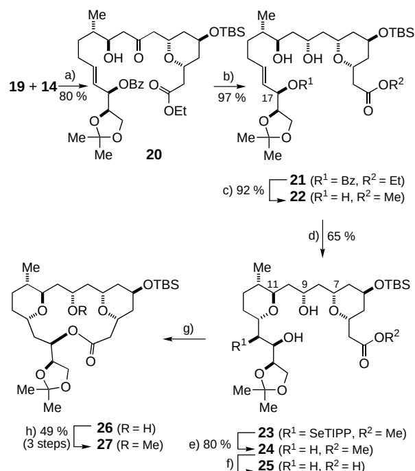
Scheme 4. a) \text{Bu}_2\text{BOTf} , \text{Et}_3\text{N} , \text{Et}_2\text{O} , -78^\circ\text{C} , then 19 , 5 h, 80 % (d.r. > 95:5); b) TABH, AcOH, \text{CH}_3\text{CN} , -40^\circ\text{C} , 70 h, 97 % (d.r. > 95:5); c) \text{K}_2\text{CO}_3 , MeOH, RT, 40 h, 92 %; d) TIPPSeBr, 2,6-di- tert -butyl-4-methylpyridine, \text{CH}_2\text{Cl}_2 , -78^\circ\text{C} , 74 % (d.r. 88:12); e) 2,4-dimethoxy-3-methyl-3- tert -butyldimethylsilylcyclohexa-1,4-diene, AIBN, n -hexane, reflux, 1 h, 80 %; f) TMSOK, \text{Et}_2\text{O} , RT, 24 h; g) 2,4,6-trichlorobenzoylchloride, \text{Et}_3\text{N} , DMAP, DMF, RT; h) \text{Me}_3\text{OBF}_4 , proton sponge, 4 Å M.S., \text{CH}_2\text{Cl}_2 , RT, 49 % (3 steps). AIBN = 2,2'-azoisobutyronitrile, M.S. = molecular sieves, proton sponge = N,N,N',N' -tetramethyl-1,8-diaminonaphthalene, TABH = tetramethylammonium triacetox borohydride, TIPP = 2,4,6-triisopropylphenyl.
